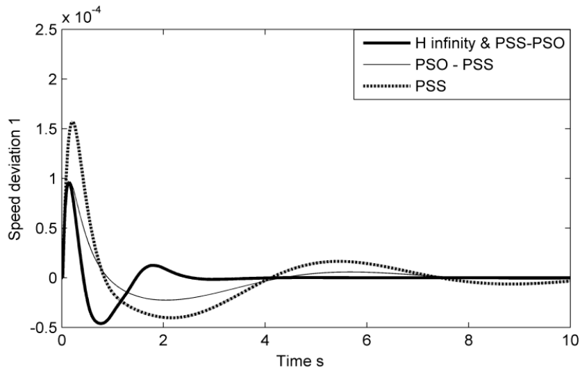
Fig. 5: Speed deviation \Delta\omega_1
