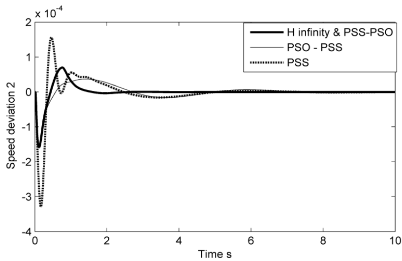
Fig. 6: Speed deviation \Delta\omega_2
