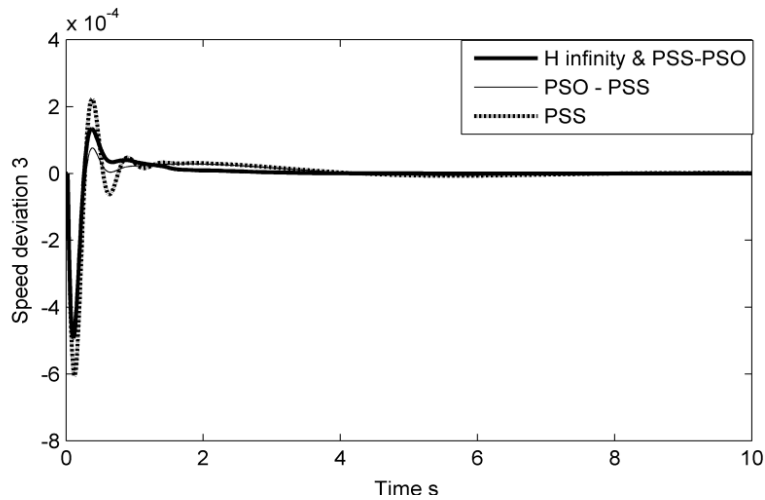
Fig. 7: Speed deviation \Delta\omega_3
