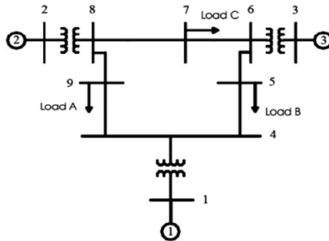
Fig. 1: Three machine nine bus power systems.
